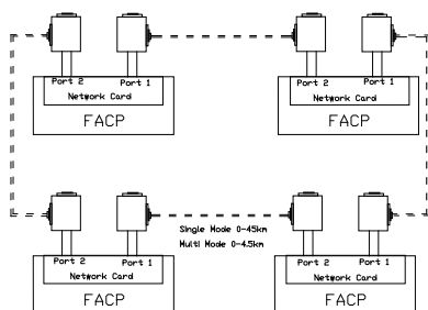
Fiber-Optic Class A network
