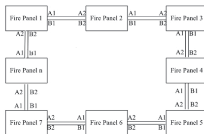
Standard Class A network
